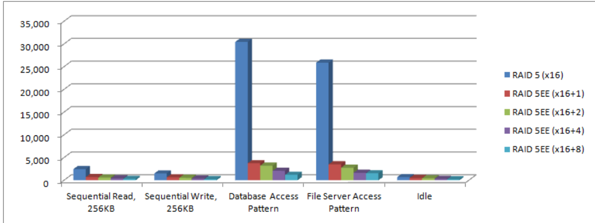
Figure 17 The Chart of RAID 5 and RAID 5EE
