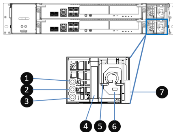
Figure 2-8 XF4226 / XN4226 Power Supply Unit Components
