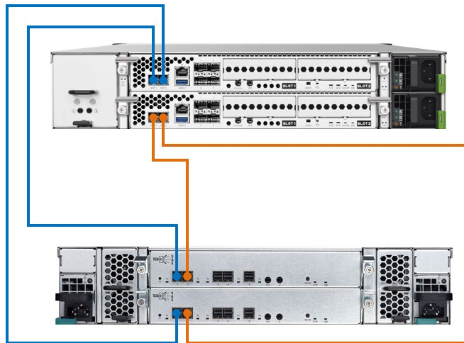
Figure 3-4 XF4226 / XN4226 Expansion Unit Connections
