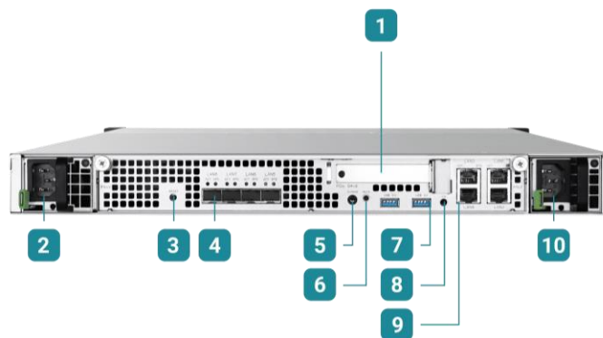
Figure 2-3 XN8104R Rear Panel Layout
