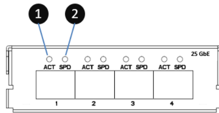
Figure 2-19 4-port 25 GbE iSCSI Host Card (SFP28) LEDs
